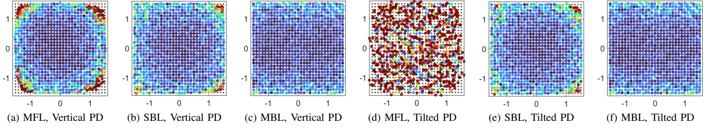
Fig. 4. Position estimation results with a vertical PD (a–c) and a tilted PD (d–f) for each configuration under the same noise level. Each estimated point is color-coded according to the positioning error, ranging from 0 cm (blue) to 8 cm (red), with values above 8 cm shown in magenta.
