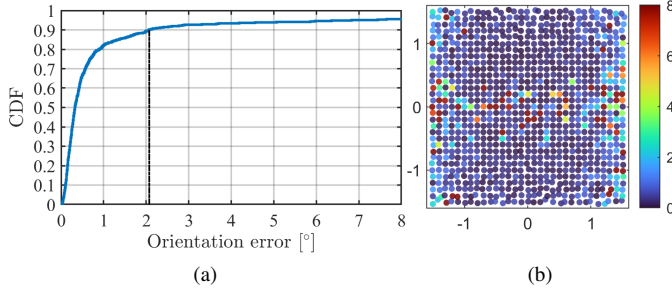
Fig. 5. Distribution of the PD orientation error: (a) CDF, (b) Heatmap.
