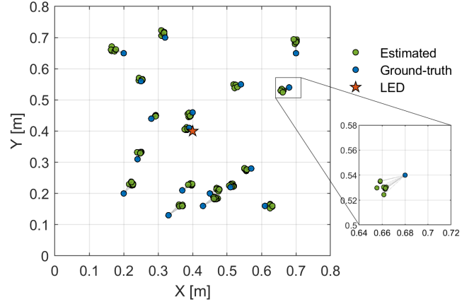
Fig. 8. Experimental 2D position estimation of the PD using the SBL configuration. For each ground-truth position, ten independent estimations were performed with different random PD tilts ranging from 0^\circ to 20^\circ .
