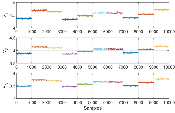
Fig. 7. Voltage samples recorded at the receiver position \mathbf{p}_r = [0.70, 0.54, 0.75] for ten different receiver orientations (represented by different colors), with a random PD tilt between 0 and 20^\circ and a random azimuth between 0 and 360^\circ .
