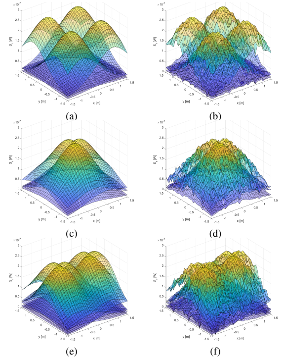
Fig. 3. RSS-value distribution in the testbed. The three rows correspond to the MFL (a,b), SBL (c,d), and MBL (e,f) configurations, respectively. For each configuration: the left subfigure shows the case when the PD is oriented vertically (a,c,e), while the right one corresponds to a randomly tilted PD of up to 20^\circ (b,d,f).
