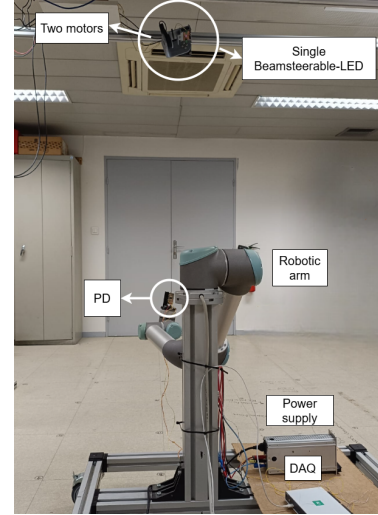
Fig. 6. Experimental setup of the mechanical SBL scenario implemented using two motors in a gimbal configuration. The receiver consists of a PD mounted on the end-effector of a robotic arm capable of both translation and reorientation of the PD.
