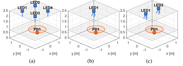
Fig. 2. Different simulation configurations: (a) MFL with 4 LEDs, (b) SBL with 3 orientations, (c) MBL with 2 LEDs and 3 orientations per LED.
