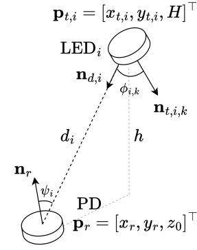
Fig. 1. Geometry of the i th ceiling-mounted LED and the PD receiver with position and orientation vectors.
